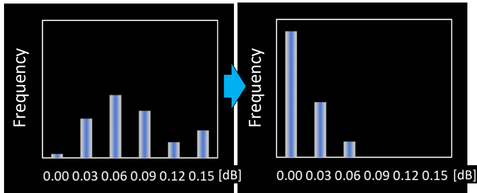
Splice loss with large cleave angle : 3 < \theta < 5 degree
